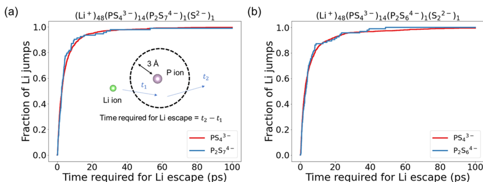
Figure 3. Fraction of Li-ion jumps counted near the \text{PS}_4^{3-} , \text{P}_2\text{S}_7^{4-} , or \text{P}_2\text{S}_6^{4-} polyanion vs the time required for Li escape from the polyanion, measured in the amorphous model structures containing (a) 14 \text{PS}_4^{3-} + 1 \text{P}_2\text{S}_7^{4-} (sample name; 1 \text{P}_2\text{S}_7 ) and (b) 14 \text{PS}_4^{3-} + 1 \text{P}_2\text{S}_6^{4-} polyanions (sample name; 1 \text{P}_2\text{S}_6 ), respectively.
