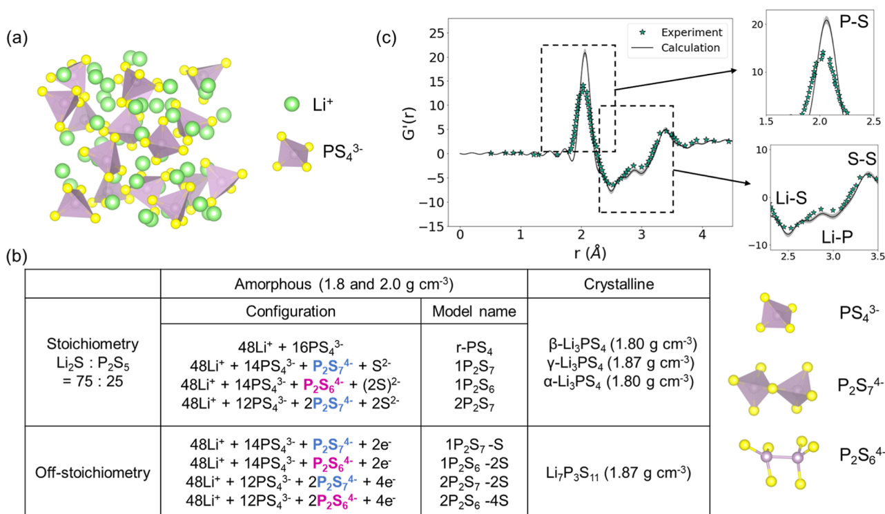
Figure 1. (a) Amorphous \text{Li}_3\text{PS}_4 structure generated by randomly distributing \text{Li}^+/\text{PS}_4^{3-} ions and melt quenching the structure at 1000 K using AIMD. (b) Poly-anion composition of amorphous \text{Li}_3\text{PS}_{4-\delta} and known crystalline phases simulated in this study. (c) Averaged neutron-weighted PDFs ( G'(r) ) of the model amorphous structures (black line, gray shade covers between maximum and minimum values) compared with that of amorphous \text{Li}_3\text{PS}_4 measured in the experiments (green stars). 16
